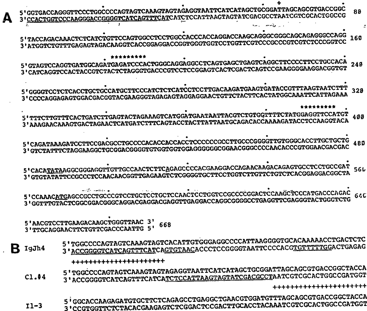
Fig 3. Sequence of t(6;14)(q31;q32) breakpoint region. (A) Nucleotide sequence of the BstEII/HpaI fragment indicated on Fig 2. Nucleotides 1 to 36 represent the Jh4 coding region underlined on the coding strand. 9 Nucleotides 39 to 63 are a putative N region. The sequence from position 64 to 668 is that of the germline IL-3 gene. 20 The IL-3 TATA box (485), transcription start (515), and initiation methionine (567) are underlined. Two proposed regulatory sequences in the promoter are marked by asterisks (positions 182 and 389). (B) Comparative sequence of the t(6;14)(q31;q32) breakpoint region. The IgJh4 region is shown with its coding region, heptamer, and nonamer underlined. Clone no. 4 is shown with putative N region sequences underlined. The IL-3 sequence is also shown. A plus sign (+) denotes the identical nucleotide between sequences. No heptamer or nonamer is identified in the IL-3 sequence.
